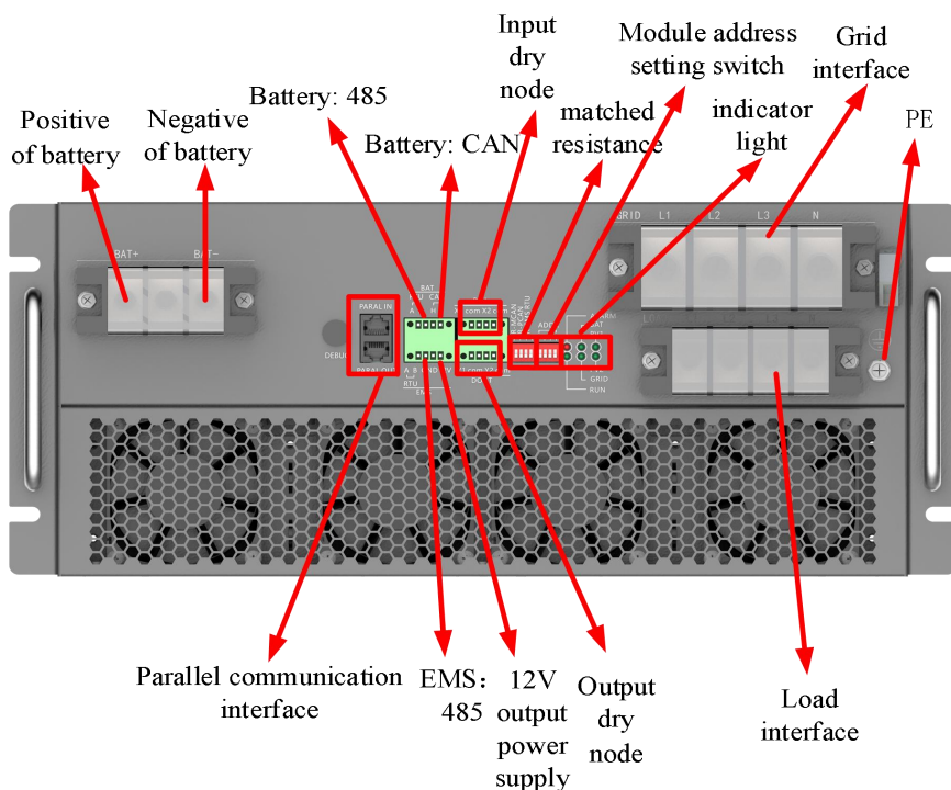
Picture 10 Port definition schematic
