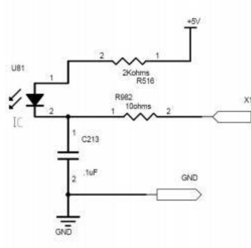
Figure 12 Internal schematic diagram of input dry node
